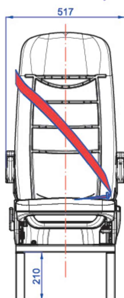
TECHNICAL DRAWING (FRONT VIEW)
