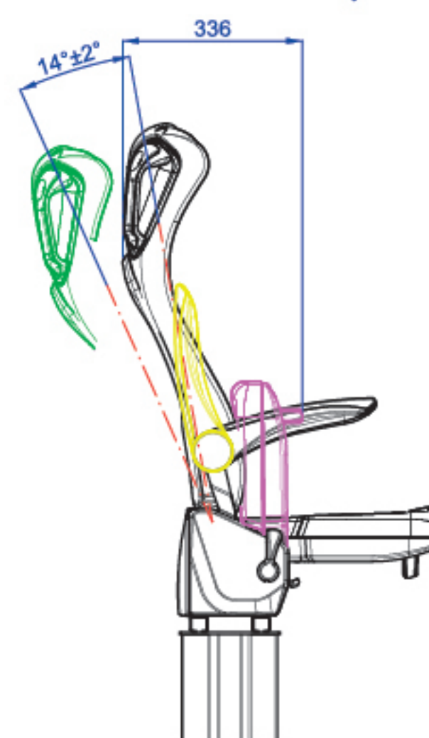
TECHNICAL DRAWING (SIDE VIEW)
