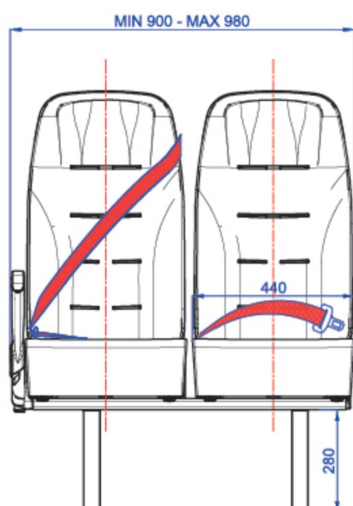
TECHNICAL DRAWING (FRONT VIEW)
