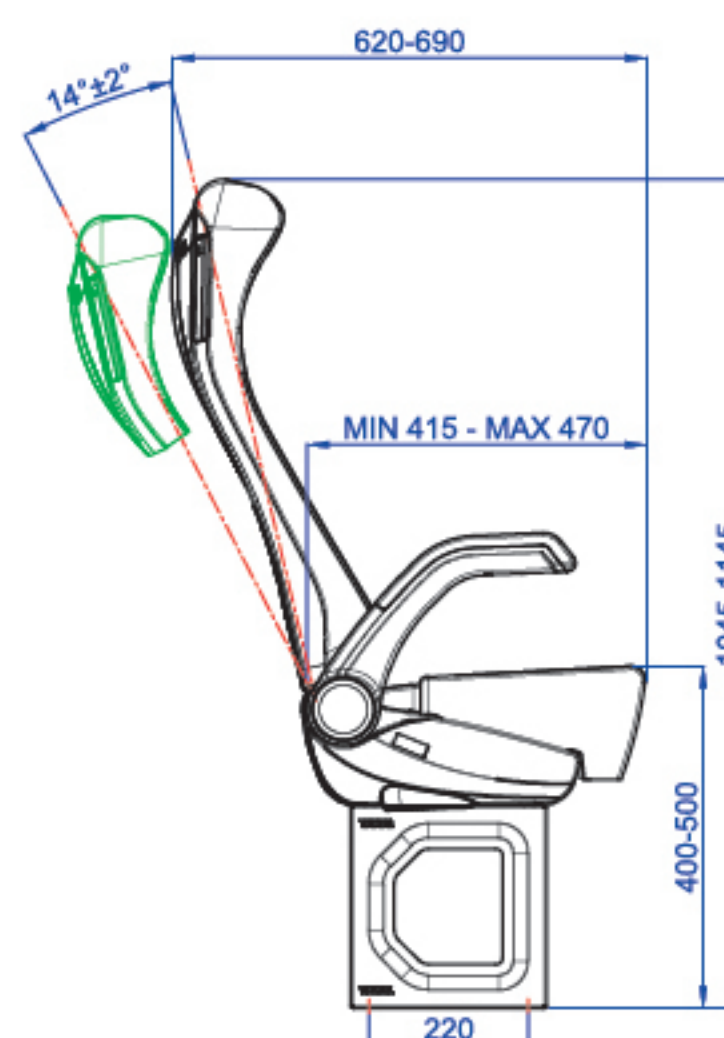
TECHNICAL DRAWING (SIDE VIEW)
